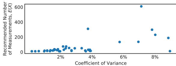
Figure 6: Relationship between CoV and \check{E}(X) .
