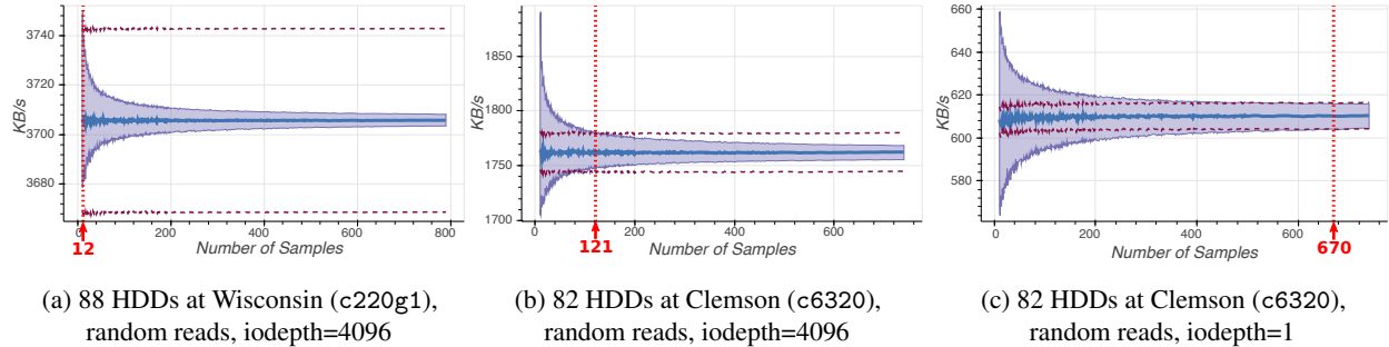
Figure 5: Nonparametric confidence intervals produced by CONFIRM. As the number of samples grows, 95% CIs (filled areas) for the medians (thick blue lines) shrink and fit within the 1% error bounds (dashed lines). This stopping condition is depicted with red lines and annotated with the numbers of recommended measurements \check{E}(X) .
