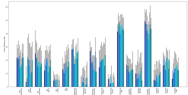
Fig. 3: Bar plot of 500 KHz steps for TX/RX pairs in Nov. 13 measurements - occupied channel.
