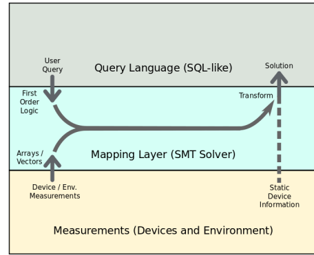
Fig. 1: WiMatch Workflow
